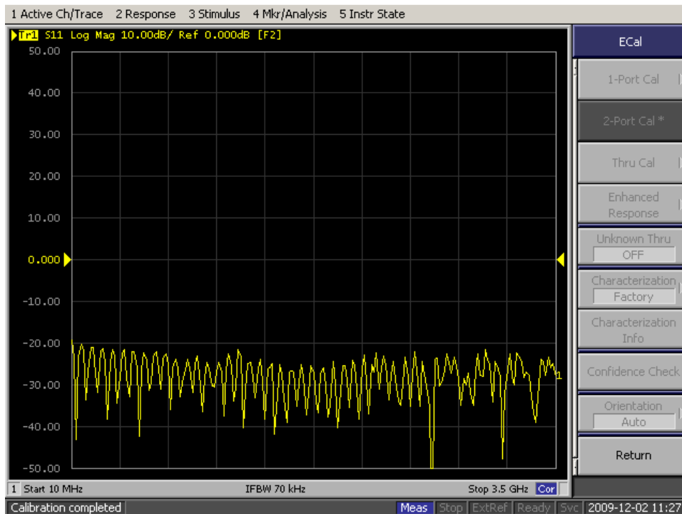
Return Loss Test Results ( Cable length : 5M)
