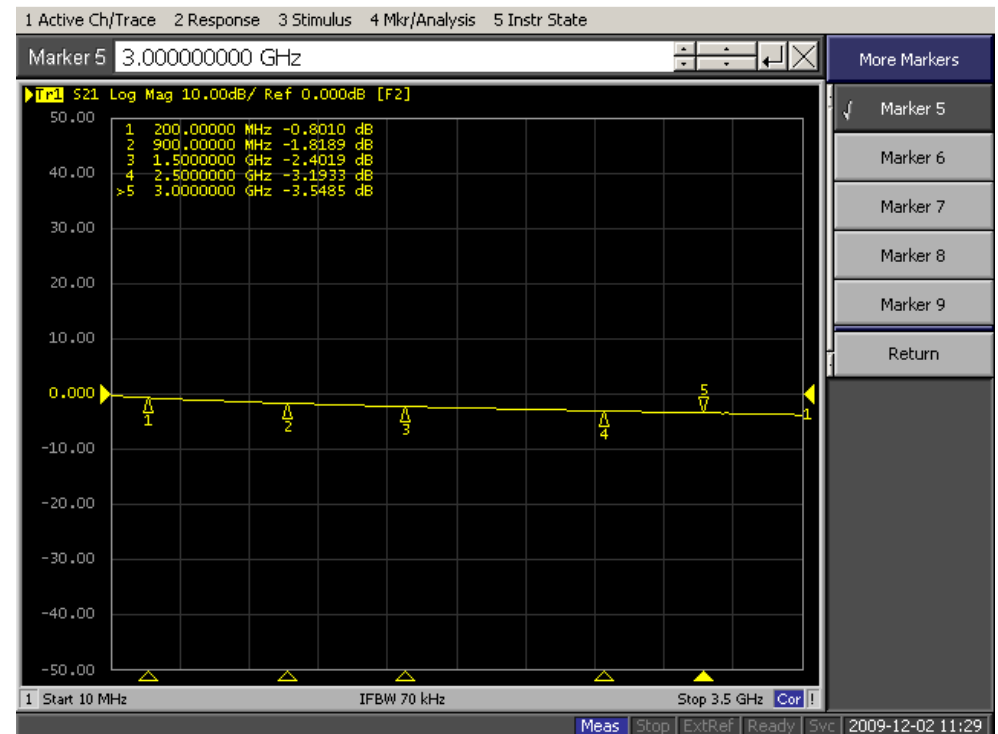
Insertion Loss Test Results ( Cable length : 5M)
