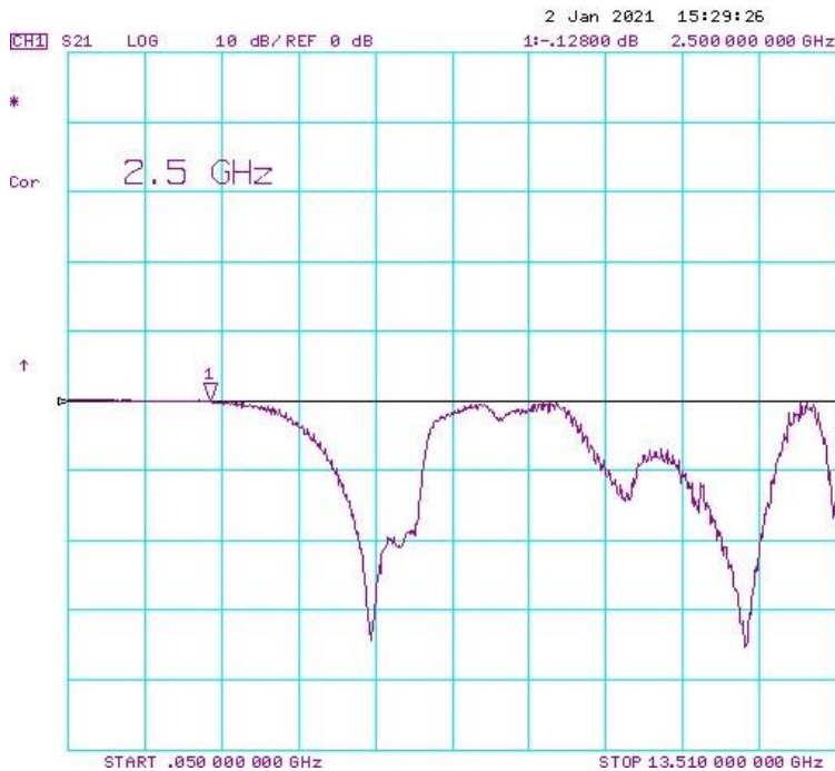
Typical insertion loss (S21)
